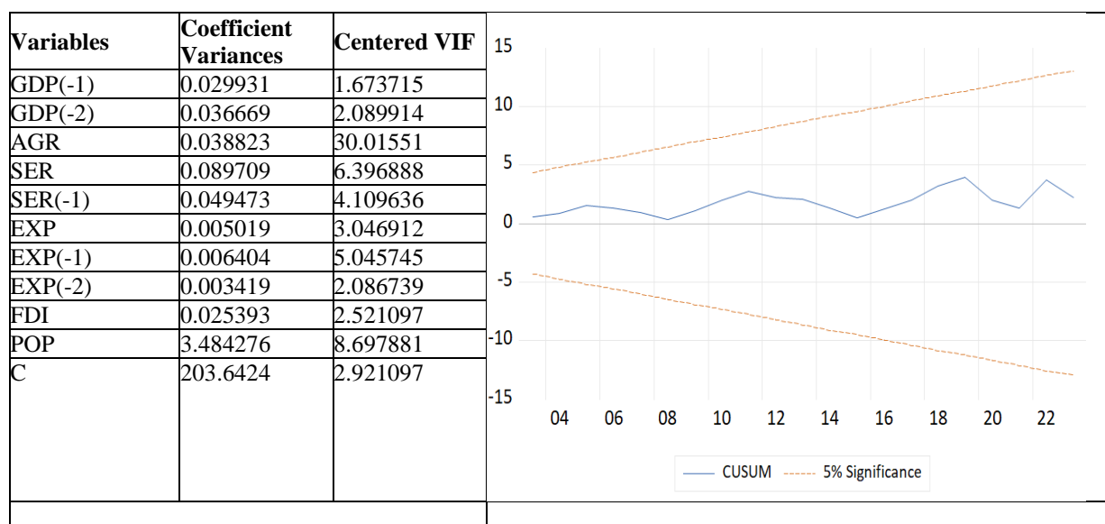
Variance Inflation Factor (VIF) and CUSUM Test Results
